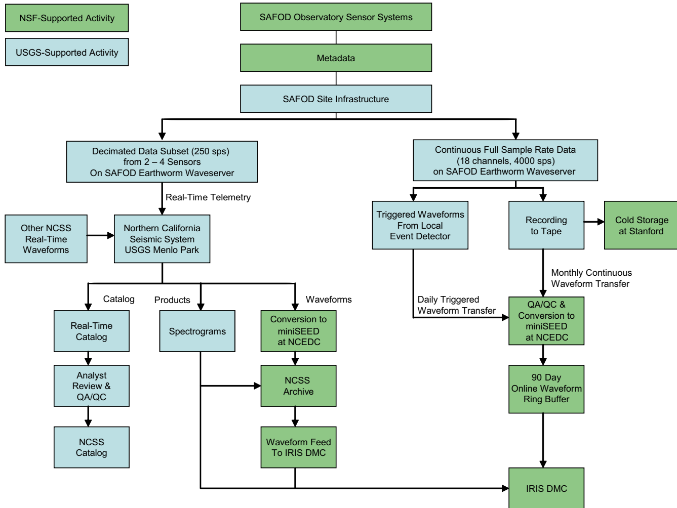
Figure 4.4. Data pathways for SAFOD seismic data. Boxes with a green background are to be supported by the EarthScope O&M budget from NSF (this proposal). Boxes with a blue background are to be supported by the USGS. The left branch of the tree follows the decimated subset of data, branching off into sections for the earthquake catalog, spectrograms, and waveforms. The catalog is a USGS product. The waveforms and spectrograms are EarthScope data products hosted at the NCEDC, which are also copied to the IRIS DMC. The right branch follows the full sample rate data through the NCEDC to the IRIS DMC. A "Local Event Detector" collects ~ 10-sec windows of full-sample-rate data, and sends those to the NCEDC on a daily basis. These files are converted to miniSEED and stored online. The tapes containing the continuous recordings are delivered to NCEDC monthly. The tapes are read and converted to miniSEED. After processing, the data are available for 90 or more days in the online ring buffer at the NCEDC and indefinitely from tape at the IRIS DMC. The field tapes are kept in storage at Stanford.
