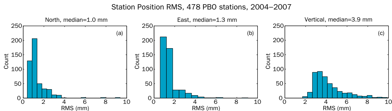
Figure 4.8. One key PBO GPS data quality metric is the RMS noise level in each station's position time series. (a) shows a histogram of the RMS noise level in the north component of the position time series for all PBO stations with at least 60 days of data through the end of January 2007; (b) shows the same, but for the east component; (c) shows the same, but for the vertical component. Median values for each are shown in the titles for each subplot. PBO is well within the range of uncertainty, less than 2 mm horizontally and 5 mm vertically, that would be expected from three years of high-quality GPS processing.
