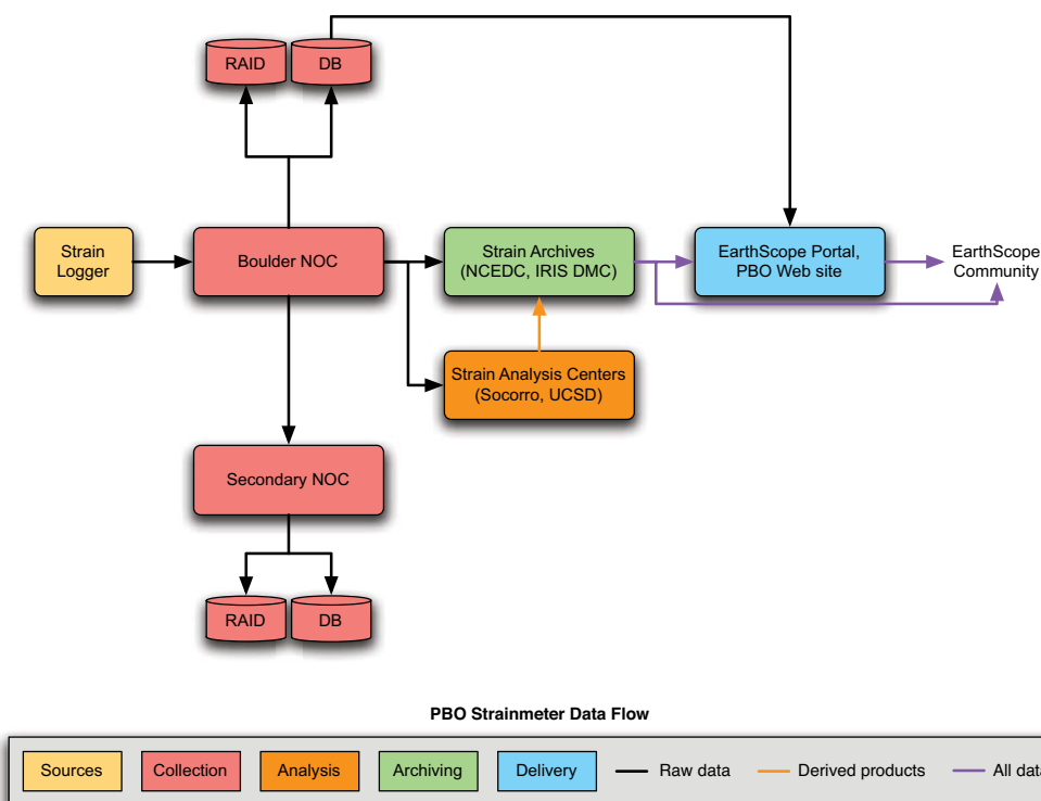
Figure 7.3. Flow of data through PBO Strain Data Management System. The Boulder Network Operations Center (NOC) downloads data from strainmeter stations, copies the data to a local RAID system, extracts necessary meta-data into the PBO Operational Database (DB), and transmits data to the PBO strain archives at the Northern California Earthquake Data Center (NCEDC) and IRIS Data Management Center (DMC). The Boulder NOC will also mirror these data to the secondary NOC on a routine basis; the secondary NOC can take over all critical operations of the Boulder NOC in the event of system failure in Boulder. The Boulder NOC also delivers data to the PBO strain analysis centers at Socorro, NM (borehole) and University of California, San Diego (laser strain), which create Level 2 products that they send to the strain archives. Users can access PBO strain data products from the archives through a number of mechanisms, as well as via the PBO Web site and the EarthScope Portal. See sections 2.3.3.5 and 2.3.3.6 for more details.
