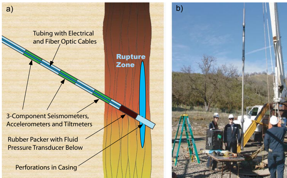
Figure 4.3. (a) Schematic of the long-term monitoring array for SAFOD. After casing is cemented in place from the bottom of corehole 3 to the surface (see Figure 3.11b), the casing is perforated in the fault zone and the array is emplaced on rigid tubing close to the target earthquake rupture zone. This array is designed so that it can be periodically removed for maintenance and repair. Unidirectional bow-springs (not shown) decentralize the seismic sensors to insure good coupling with the casing, and a rubber packer is inflated just above the perforations to monitor variations in fluid pressure during the earthquake cycle. (b) Photograph of engineers from Pinnacle Technologies testing a prototype for the seismic and tilt sensors in the SAFOD borehole following Phase 2 drilling.
