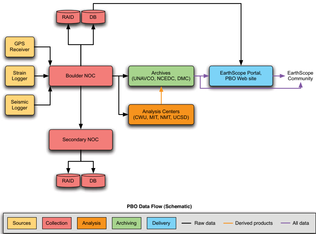
Figure 4.7. Flow of data through PBO Data Management System. The Boulder Network Operations Center (NOC) downloads PBO data, mirrors them to a secondary offsite NOC, and transmits them to archives and analysis centers. PBO analysis centers analyze raw data and produce a variety of Level 2 data products (Table 4.2). PBO archives archive and distribute PBO data products to end users directly and via the PBO Web site and EarthScope Portal. Either NOC can provide critical data flow control functions; either archive can receive, archive, and distribute data products; and analysis can be done with only one operational Analysis Center. Redundant, geographically distributed data collection centers and archives ensure high reliability and availability of data products despite possible system failures at any one center.
