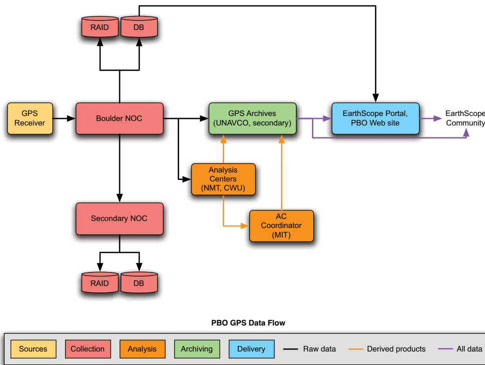
Figure 7.2. Flow of data through PBO GPS Data Management System. The Boulder Network Operations Center (NOC) downloads data from GPS stations, copies the data to a local RAID system, extracts necessary meta-data into the PBO Operational Database (DB), and transmits data to the UNAVCO Facility Archive and the secondary NOC. Data flow to the GPS Analysis Centers for processing, and all data products flow to the UNAVCO Facility Archive and an offsite backup archive for archiving and delivery to end users. Either NOC can provide critical data flow control functions; either archive can receive, archive, and distribute data products; and analysis can be done with only one operational Analysis Center. Redundant, geographically distributed data collection centers and archives ensure high reliability and availability of data products despite possible system failures at any one center. See section 2.3.3.1 for more details on the Boulder NOC, 2.3.3.3 for the roles of the GPS Analysis Centers, and 2.3.3.4 for details on the UNAVCO Facility Archive.
