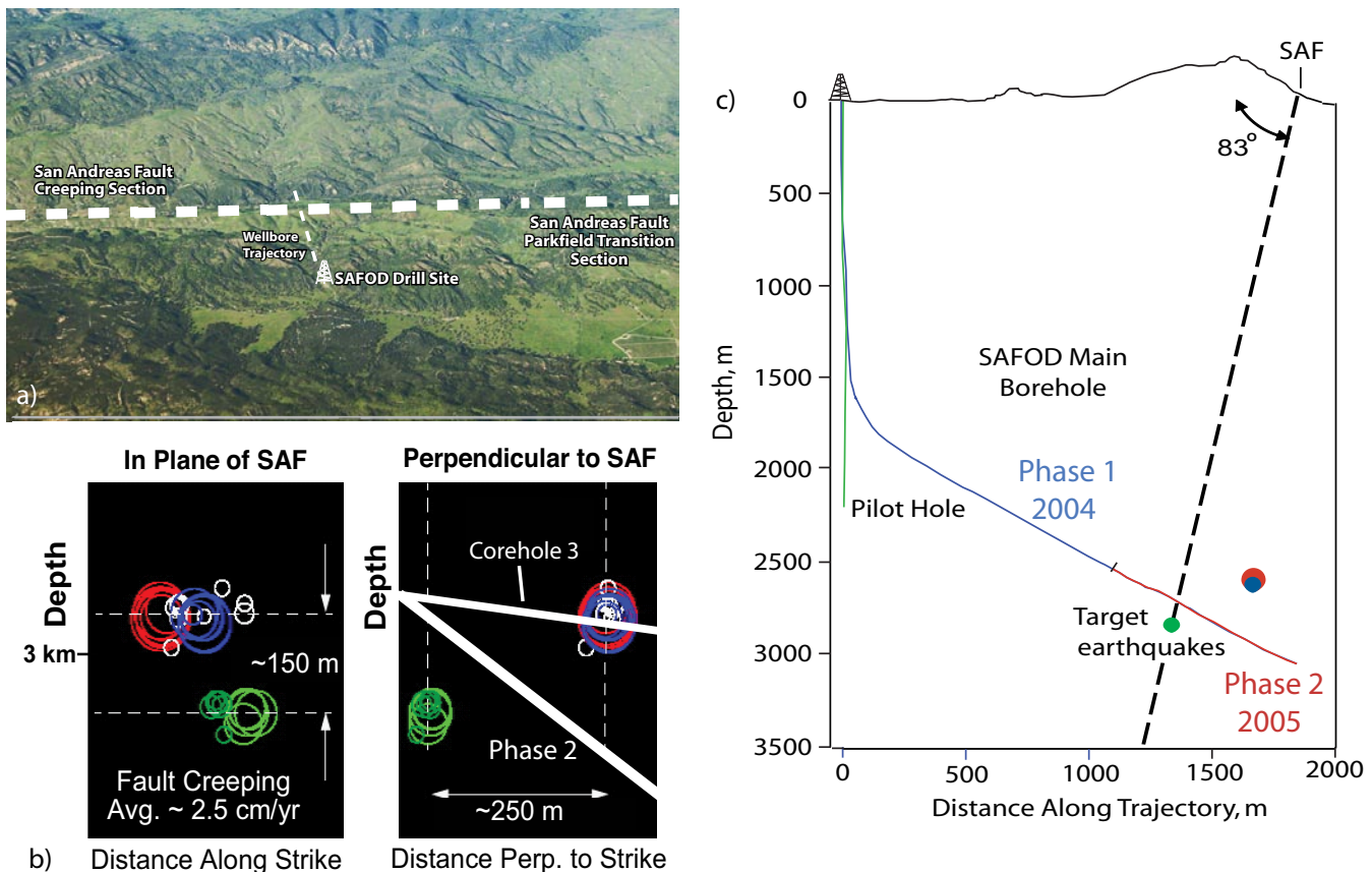
Figure 3.11. (a) SAFOD is located in central California where slip on the San Andreas Fault occurs mostly by fault creep with isolated, small “fault patches” produce repeating microearthquakes. The drill site is located at the southeastern end of the creeping section of the San Andreas, where the surface creep rate begins to gradually decrease in the Parkfield section of the fault. (b) The targets for SAFOD drilling are repeating microearthquakes at ~3 km depth. As can be seen in the figure, there are three groups of repeaters in the target area. As shown in the cross section in a plane parallel to the San Andreas, the groups of repeaters shown in red, blue, and green correspond to M \sim 2 earthquakes that recur every ~2.5 years. As shown in the cross section perpendicular to the fault, the red and blue repeaters occur on a different strand of the fault than the green repeaters. Hence, there are multiple active fault traces at depth. The white lines schematically illustrate the location of the SAFOD main borehole—drilled in the summers of 2004 and 2005—and a corehole targeting the microearthquakes to be drilled in 2007. (c) Trajectories of the SAFOD pilot hole, drilled in 2002, and the SAFOD main hole. The microearthquake locations are to the southwest of the surface trace of the San Andreas Fault.
