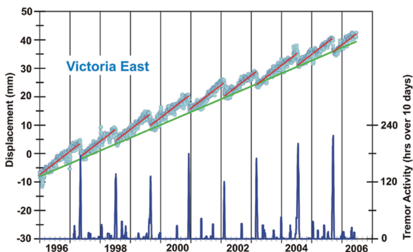
Figure 3.10. Summary of geodetic and seismic observations that characterize episodic tremor and slip in the Pacific Northwest. Blue circles show daily changes in the east component of the position of the CGPS station ALBH (Victoria, B.C.) The green line indicates the long-term eastward linear trend of motion ( \sim 4 mm/yr) due to margin deformation caused by the locked portion of the subduction interface. The red line segments show the average linear motion ( \sim 8 mm/yr) over \sim 15 -month segments due to temporary additional plate coupling on a deeper portion of the plate interface. This deeper coupling is released over periods of weeks every 15 months, resulting in repeated temporary westward motion and the characteristic sloped sawtooth time series. The bottom graph shows the total number of hours of tremor activity in a sliding 10-day period. With a high density of CGPS stations and strainmeters in the Pacific Northwest, PBO will provide critical data to elucidate the mechanism of ETS and understand its implications on seismic potential at subduction zones. Courtesy of Herb Dragert.
