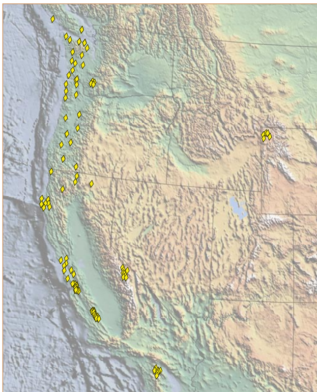
Figure 4.9. Map showing locations of PBO borehole strainmeter stations.
