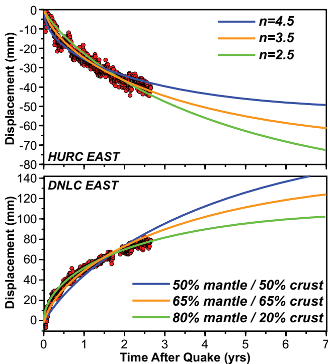
Figure 3.9. Red dots show position time series (east component) for two continuous GPS stations installed in Alaska after the Mw7.9, 2002, Denali earthquake, now part of PBO. Solid lines show fit and predicted continuation of a postseismic relaxation signal for ranges of models that acceptably fit the existing data. Upper panel illustrates the role of power-law parameter n , which controls the time dependence of viscoelastic relaxation assuming a stress-dependent rheology. Lower panel shows the contribution of upper mantle vs. lower crust to the relaxation signal. All models show that the Denali postseismic signal is likely to last for years into the Earthscope O&M phase. The next few years of data at PBO sites in Alaska will greatly constrain the range of possible models.
