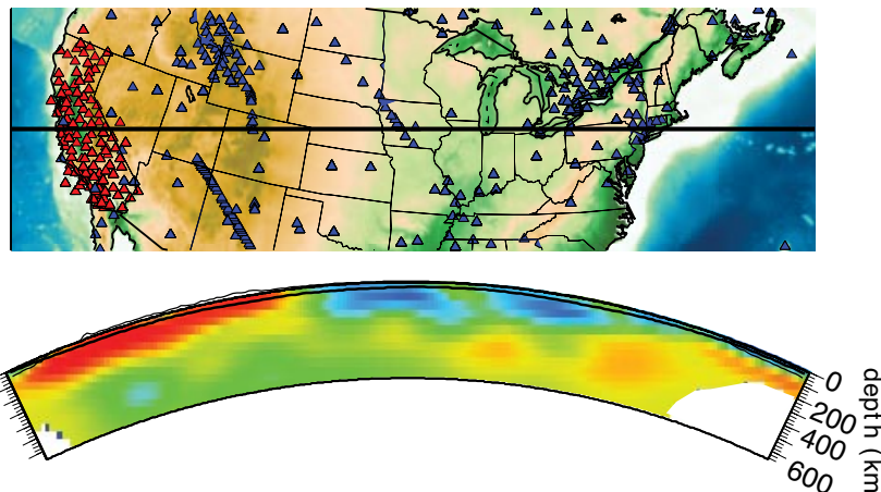
Figure 3.3. Example of lithospheric and asthenospheric scale imaging achieved by surface wave analysis using ANSS Backbone and USArray Transportable Array recordings. This is a cross section through a tomographic model for the North American upper mantle. The western United States is much better illuminated than the central and eastern United States because of data provided by USArray Transportable Array stations (red triangles). As the Transportable Array is fully deployed and migrates eastward, the entire lithosphere and asthenosphere under the contiguous United States will be imaged at high resolution. Courtesy of S. van der Lee.
