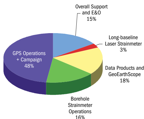
Figure 5.2. An overview of weighting of the major WBS elements (legs) for the first five years of the PBO Operations and Maintenance Project.
