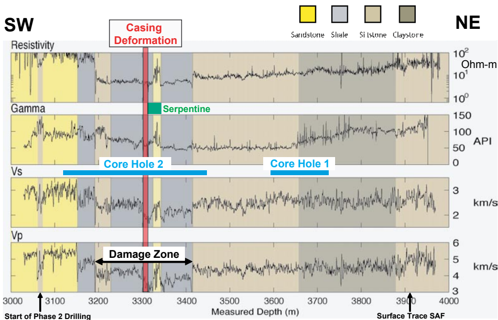
Figure 3.13. Geophysical well logs acquired across the San Andreas Fault Zone during SAFOD Phase 2, superimposed on major lithologies derived from cuttings analysis. Depths are as measured along the borehole, which is inclined at an angle of 54-60° from the vertical (see Figure 3.11c for reference). Also shown are zones of casing deformation revealed by repeat multi-finger caliper logging (corresponding to an active trace of the San Andreas Fault at a measured depth of ~3300 m) and an ~200-m-wide damage zone defined by anomalously low P- and S-wave velocities and resistivity. X-ray diffraction analyses on cuttings reveal the occurrence of serpentine (shown in green) and talc just to the northeast of the casing deformation zone, which is perhaps responsible for the low strength and predominately creeping behavior of the fault at this location. The approximate locations of two out of the three multilateral core holes planned for SAFOD Phase 3 are shown in blue. These core holes will be placed as close as possible to the trajectory of the Phase 2 borehole to sample two major faults identified from well logs, casing deformation, cuttings analysis, fault-zone guided waves and microearthquake relocations. A third core hole (not shown) will be steered away from the main SAFOD borehole to obtain core samples from directly within one of the rupture zones of the M~2 earthquakes shown in Figure 3.11.
