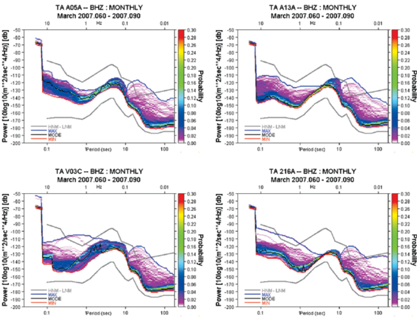
Figure 4.13. Examples of the noise performance (power spectral density plots) for typical Transportable Array stations. The range of noise levels over a one month time interval is shown. The brighter colors indicate the most probable levels; outliers indicate less frequent changes in signal level due to wind, traffic, or earthquakes. The microseismic peak near 8 sec is typical of continental stations. The noise levels over the entire range shown compares favorably with the performance of other permanent stations of the GSN and ANSS.
