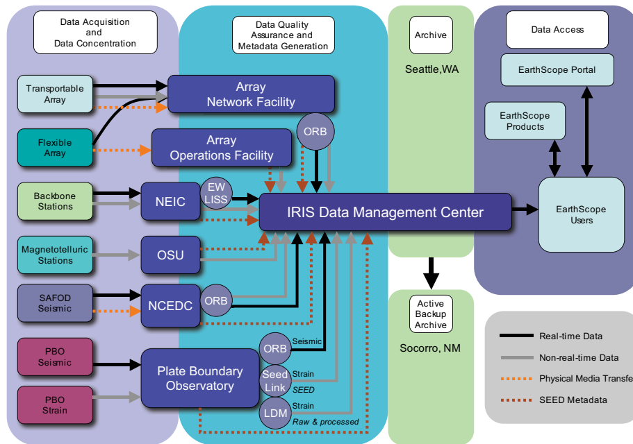
Figure 4.17. Dataflow within the Data Management System. This figure shows the variety of sources that send their data to the IRIS DMC from EarthScope sources. These include strain and seismic data from PBO, high-rate seismic data from SAFOD, magnetotelluric data from USArray, as well as seismic data from the Reference Network, Transportable Array, and Flexible Array. Data flow is complex and reaches the DMC from six different facilities using a variety of communication protocols.
