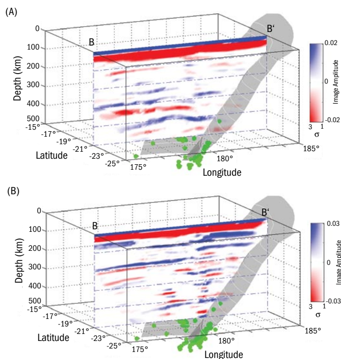
Figure 3.5. An example of use of USArray Transportable Array, ANSS Backbone, and broadband regional network data to study upper mantle structure far from North America. These are east-west vertical cross sections showing reflections in the upper mantle wedge above the Tonga Slab (gray facade). P wave reflectivity is shown in the upper panel, and SH reflectivity is shown in the lower panel. Deep focus events used as sources are shown as green dots. The arrivals are underside reflections observed at teleseismic distances as precursors to surface reflections pP and sS. These are imaged by migrating signals from North America and other global broadband stations. The blue stripes indicate reflections from impedance increases with depth, while red stripes are from impedance decreases with depth. The blue stripes at the surface are from the pP and sS reflections, which have a side-lobe giving the underlying red bands. Remarkable, unexpected reflectivity is observed in the mantle wedge. Courtesy of Y. Zheng, Y. T. Lay, M. P. Flanagan, and Q. Williams.
