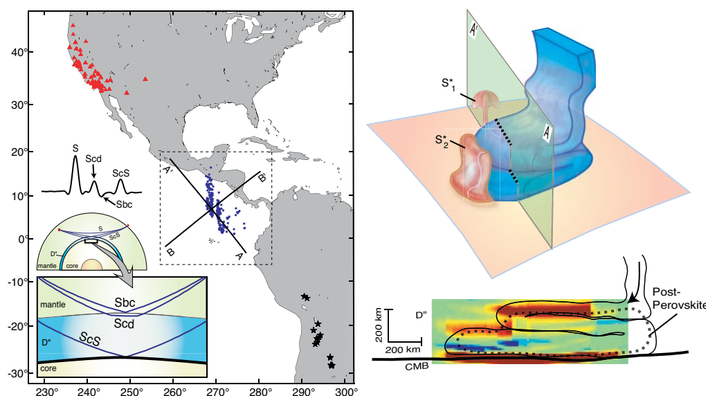
Figure 3.6. An example of use of USArray Transportable Array and broadband regional network data to study lower-most mantle structure below North America. The deep mantle corridor sampled by paths from deep South American events to the initial Transportable Array deployment in the western United States is shown on the left. S and ScS observations were migrated to form the image on the right along profile A'-A, which is interpreted as having a reflector above the core-mantle boundary caused by post-perovskite phase transition in a cold, folded and piled relic Farallon slab. From: Hutko, A. R., T. Lay, E. J. Garnero, and J. Revenaugh. 2006. Seismic detection of folded, subducted lithosphere at the core-mantle boundary. Nature 441:333-336.
