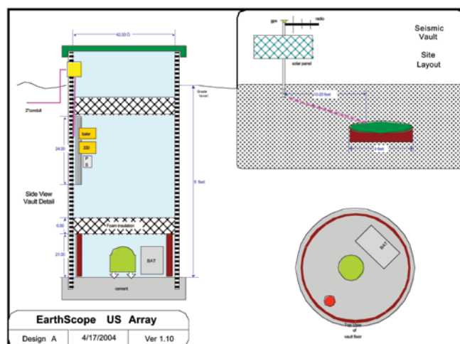
Figure 4.14. Details of the standard site vault developed for Transportable Array stations. Photographs of installation and sites are shown in Figure 2.2.
