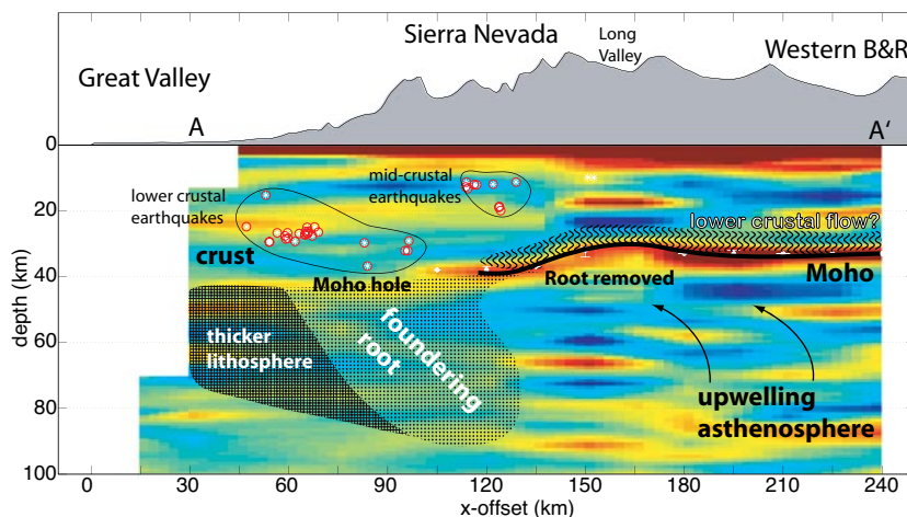
Figure 3.2. Example of deep crust and uppermost mantle imaging achieved by passive-source seismology using portable deployments of USArray Flexible Array instruments (SNEP project). This is a southwest-northeast oriented cross section across the Sierra Nevada with receiver functions and interpretations. Surface topography along this profile is plotted along the top of the cross section. Red colors correspond to positive polarity arrivals while blues mark negative polarities. Earthquakes located near this profile are plotted as white asterisks within red circles. An interpretation of flow within the lower crust is based on observations of anisotropy at the base of the crust towards the eastern part of the array (Frassetto et al., 2006). The lack of a Moho arrival along the southwestern portion of the cross section can be explained by a gradual increase in seismic velocities between the base of the crust and the still-intact portion of the batholithic root. The bright Moho present to the northeast marks the sharp contrast between the crust and inflowing asthenosphere that replaces the root following removal. Courtesy of H. Gilbert, C. Jones, and G. Zandt.
