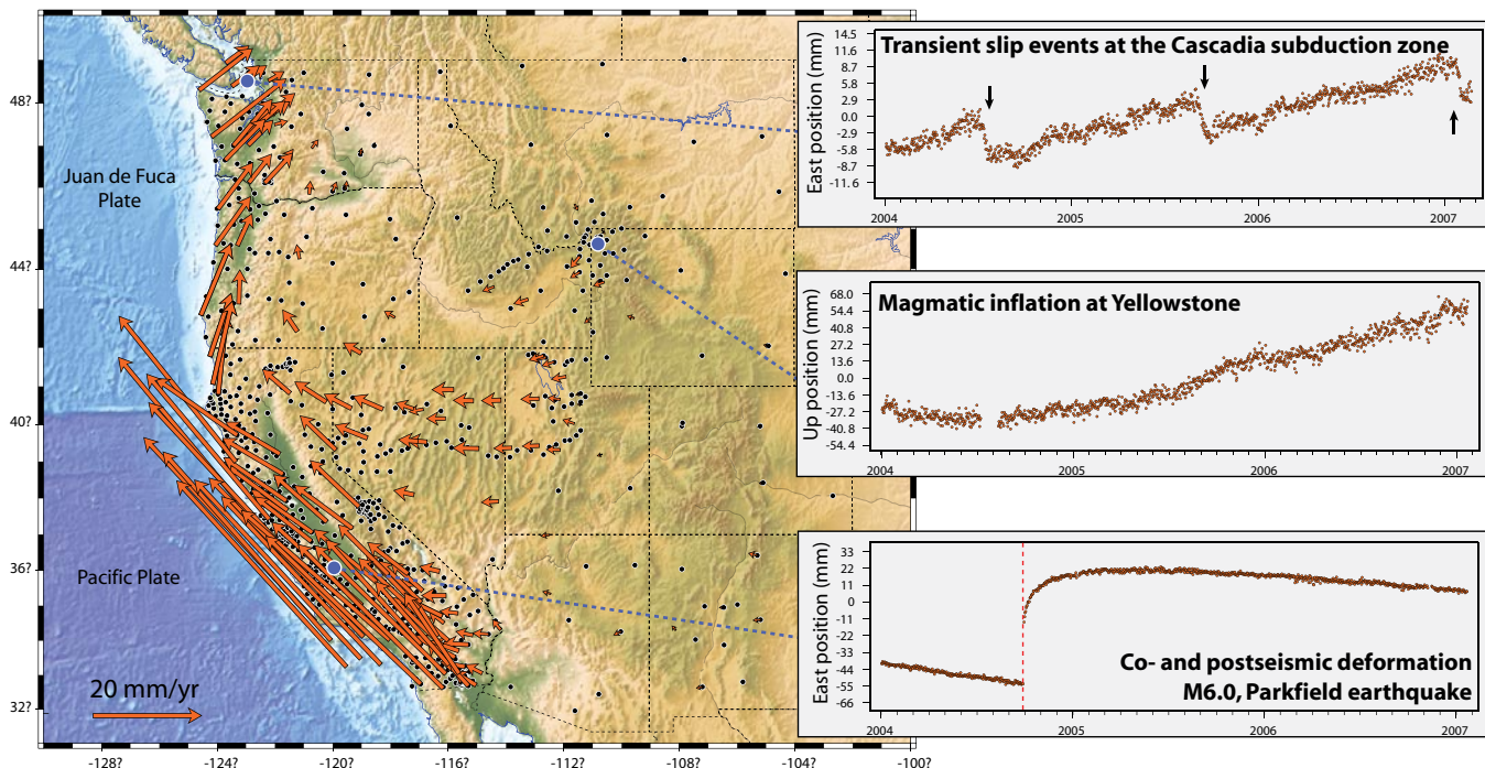
Figure 3.7: The PBO GPS network is already providing outstanding data to elucidate the dynamics of plate boundary zone, subduction, and earthquake and magmatic processes in the western United States and Alaska. Red arrows on the left panel show PBO site velocities with respect to stable North America (for a sake of readability, only a subset of the 708 sites currently processed by the analysis centers are shown). Block dots show the location of all PBO sites. Right panels are time series of daily position at three sites, illustrating transient signals. Top panel shows slow slip events on the Juan de Fuca/North America subduction in the Pacific Northwest ("ETS events"). Center panel shows recent uplift in the Yellowstone area due to magmatic activity. Bottom panel shows co- and postseismic deformation associated with the 2004, M6.0, Parkfield earthquake. Courtesy of Eric Calais.
