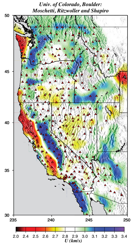
Figure 3.4. Example of crustal- and lithospheric-scale structure imaged by ambient noise tomography using USArray Transportable Array and ANSS Backbone recordings. This is a surface wave tomography map for 16-second-period Rayleigh wave group velocity, where warm shades are slow and cool shades are fast. More than two years of Transportable Array data (stations shown as red triangles) were used to construct this image. Courtesy of M.P. Moschetti, M.H. Ritzwoller, and N.M. Shapiro.
