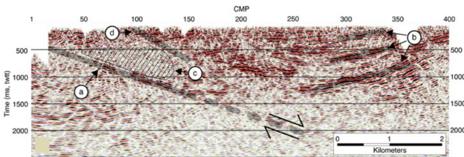
Figure 3.1. Example of high-resolution shallow crustal structure imaging achieved by active-source seismology using portable deployments of USArray Flexible Array and other instruments. This migrated image of the Surprise Valley basin near the NV-CA-OR border has no vertical exaggeration based on basin-fill V_p=2 km/s. Common mid-point spacing is 20 m. The Surprise Valley Fault (SVF) (a) forms a continuous, moderate-amplitude low-angle east-dipping reflection that bounds the western side of the basin. Prominent west-dipping reflections (b) on the eastern edge of Surprise Valley correspond to late Miocene to Pliocene (8–3 Ma) volcanic strata. The reflection-free region (c) immediately above the SVF is interpreted as alluvium deposited along the range-front during footwall exhumation. West-dipping reflections near CDP100 appear to be truncated by a fault splay (d) above the SVF. Courtesy of D.W. Lerch, S.L. Klempere, A. Egger, and J.P. Colgan.
