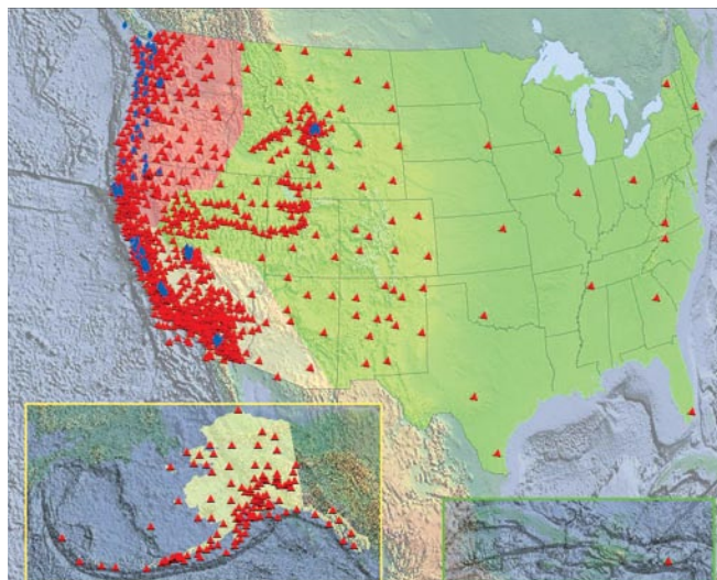
Figure 4.10. PBO GPS (red triangles) and strainmeter (blue triangle) instrumentation footprint. Map color coding indicates approximate division of resources for O&M. Alaska area is shown in light green and will be serviced out of the Anchorage, AK office. Red shading shows stations maintained out of the Portland, OR main office and Ellensburg, WA and Eureka, CA home offices. Blue shading shows stations maintained out of the Southern California office and a home office in San Francisco. Large green shading indicates stations maintained out of home offices in either Reno or Salt Lake City, Bozeman, MT, and UNAVCO Boulder.
