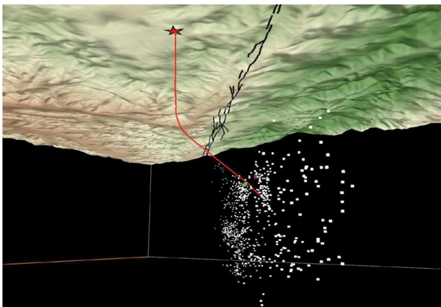
Figure 3.12. Seismicity of the San Andreas Fault as seen from a vantage point in the earth looking to the northwest. Hypocenters were determined by the Parkfield Area Seismic Observatory (PASO) UNO, PASO DOS, and EarthScope Flexible Array (PASO TRES) experiments, courtesy of Steve Roecker (RPI) and Cliff Thurber (University of Wisconsin). The San Andreas Fault is made visible by more than 1000 microearthquakes observed by the PASO networks. The SAFOD main hole is shown in red, extending downward from the surface facility (star). The surface trace of the fault is shown in black draped over the topography. The absolute locations of the SAFOD target earthquakes (red, blue and green symbols) were determined using travel time observations from instruments in the SAFOD main hole; PASO TRES, U.C. Berkeley HRSN and USGS NCSN network data; and active-source seismic experiments (recorded downhole and on the surface networks) conducted in 2004, 2005, and 2006.
