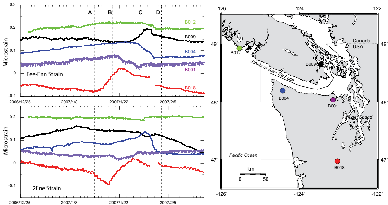
Figure 2.3. A strain transient moves from north to south through the PBO strainmeter network due to propagating transient slip along the Cascadia subduction zone. Left subfigures show shear strain recorded by PBO borehole strainmeters located in the Pacific Northwest (see map at right), from December 25, 2006 to February 20, 2007. Data have been detrended and tides and atmospheric pressure have been removed. Dotted lines show the stages of the 2007 ETS tremor. (A) tremor is detected in central Puget Sound. (B) tremor is detected in the northern Puget Sound. (C) tremor migrates across the Straits of Juan de Fuca. (D) tremor ceases.
