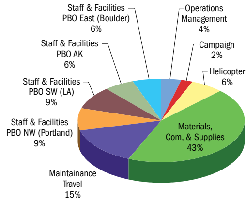
Figure 5.7. GPS operations.
