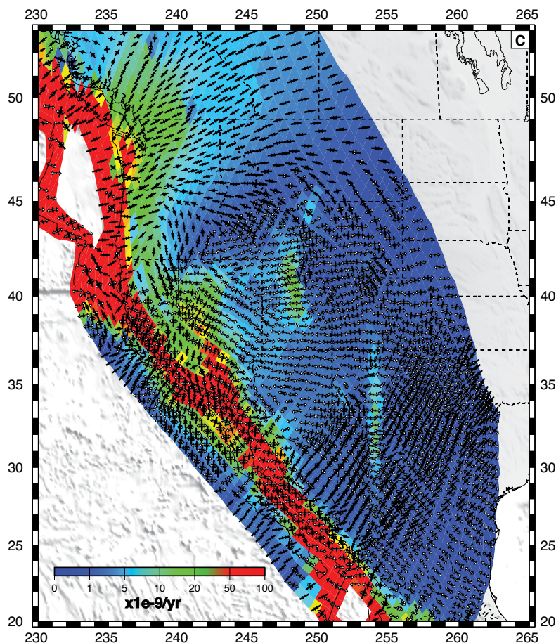
Figure 3.8: Strain rate field in the western United States derived from existing GPS velocities. Background color shows strain rate magnitude, solid and white bars show extensional and compressional principal axis, respectively. This preliminary description of the strain rate field across the western United States will be greatly improved as PBO delivers reliable GPS velocities at more sites, allowing researchers to investigate the mode of deformation of continents and the forces driving plate-boundary-zone deformation. Courtesy of Lucy Flesch.
