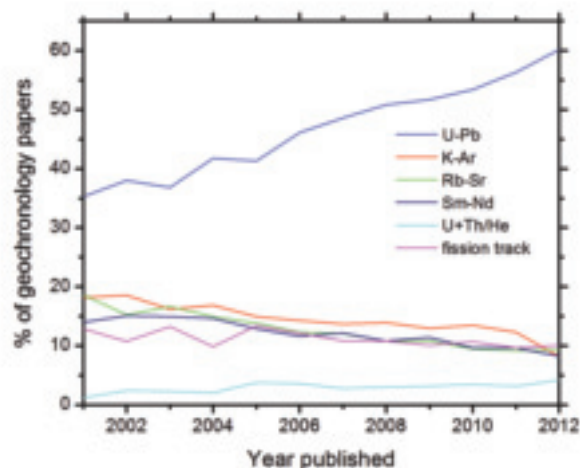
Figure 3 From 2001 to 2012, as the number of Geochemistry and Geophysics papers increased by 76%, U-Pb rose from 35% to 60% of the total in the Geochemistry & Geophysics category, implying that reporting of most other methods is declining. (Web of Science).
